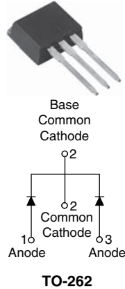
30CTH02-1PbF
