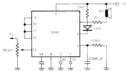
Figure 12: Connections for Unused Inputs and Loudspeaker Output.
