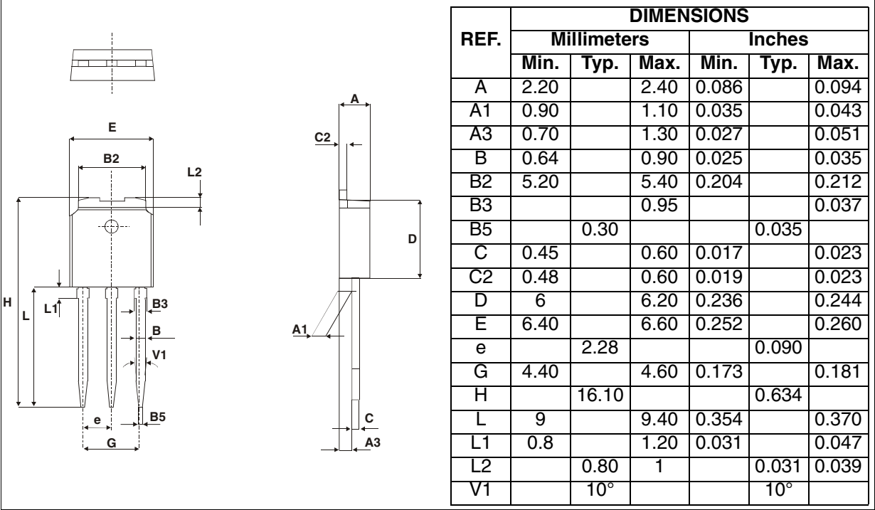
Figure 20: IPAK Package Mechanical Data
