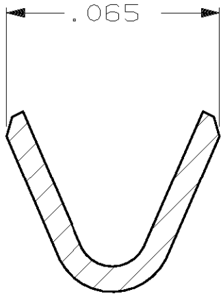
SECTION Y-Y WIRE BARREL SCALE 25:1
