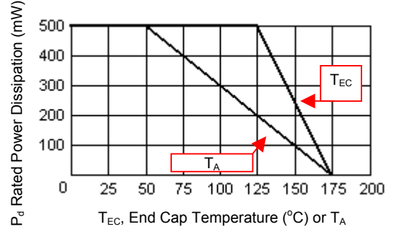
FIGURE 2 Power Derating Curve
