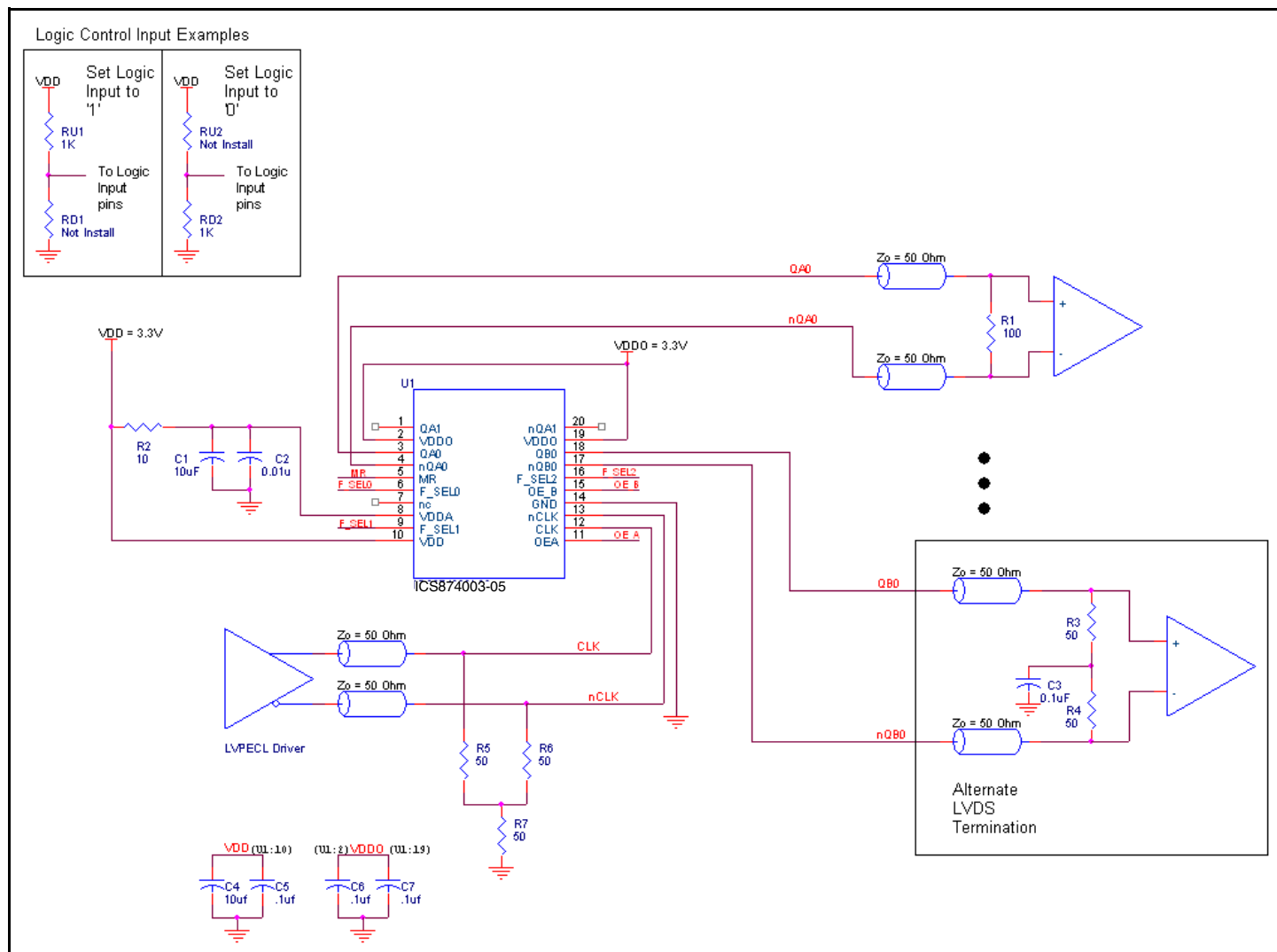
Figure 5. ICS874003-05 Schematic Example
