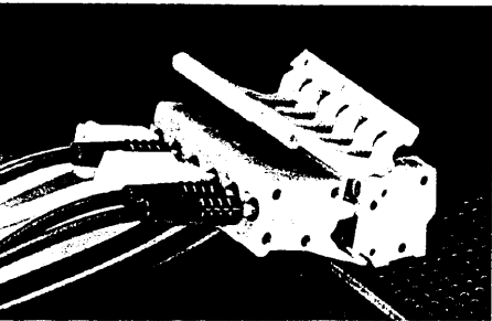
Testing on terminal blocks with connected wires. Maximum connectable wire size at 0-196/0-2 in (5/5.08 mm) pitch: AWG 16 (1.5 mm²)
