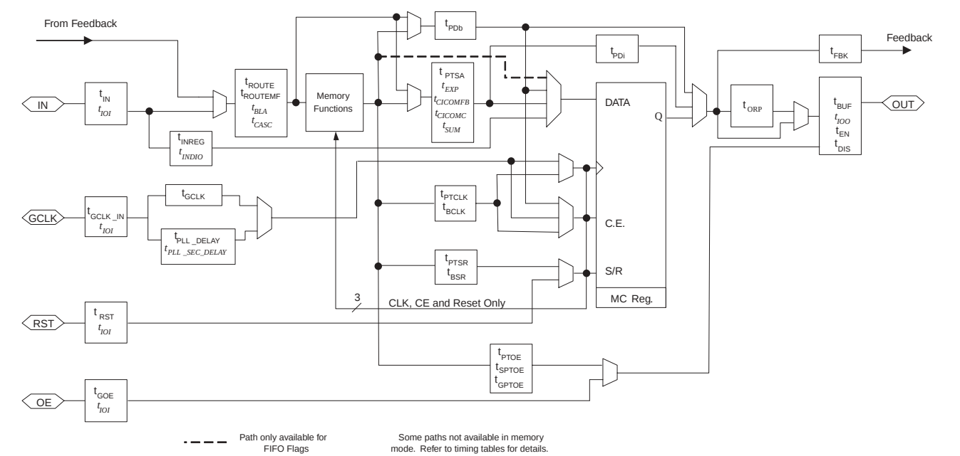
Figure 20. ispXPLD 5000MX Timing Model Diagram
