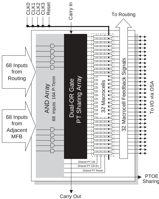
Figure 3. MFB in SuperWIDE Logic Mode
