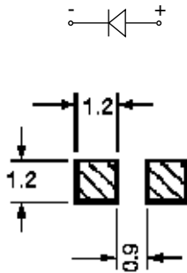
Suggested pad dimensions for reflow soldering
