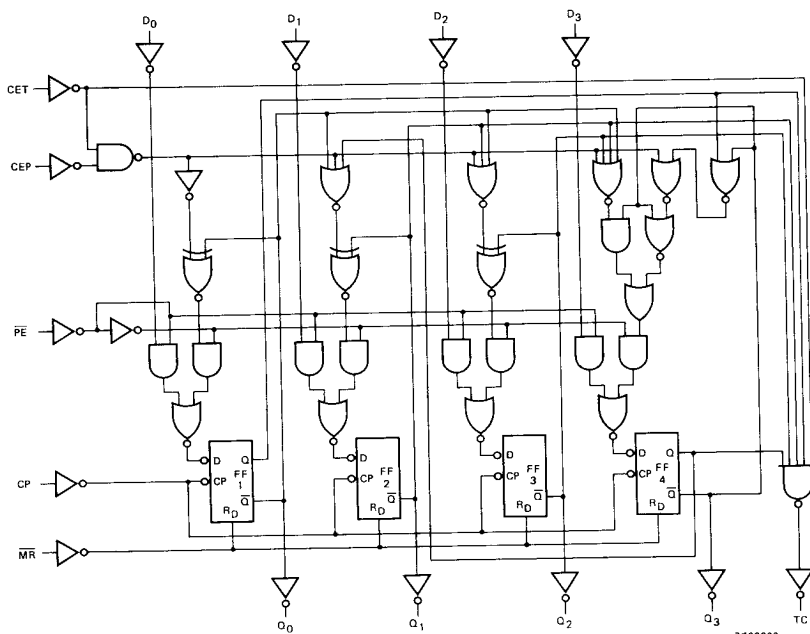
Fig. 7 Logic diagram.
