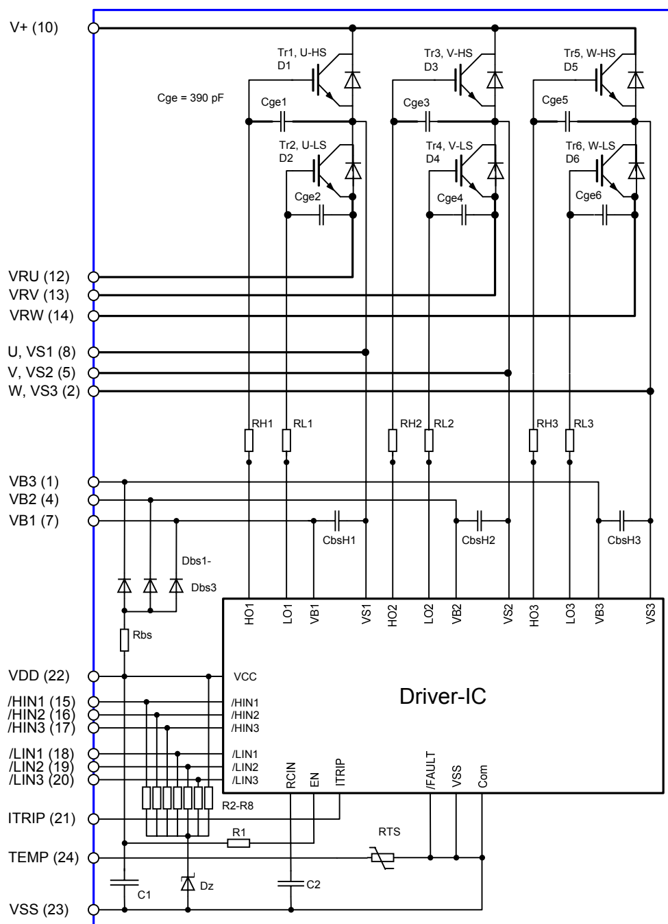
Figure 1: Internal Schematic
