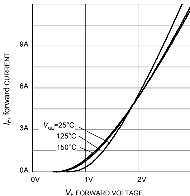
Figure 6. Typical diode forward current as a function of forward voltage
