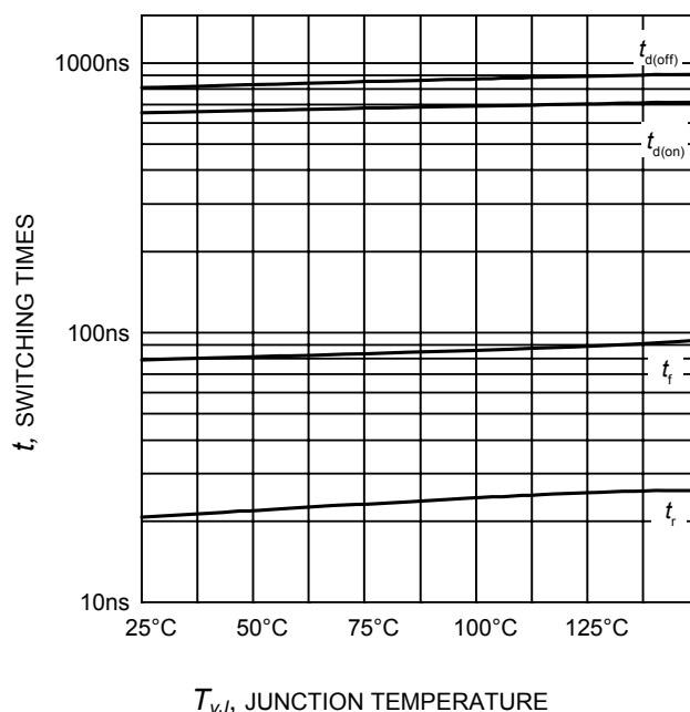
Figure 8. Typical switching times as a function of junction temperature (inductive load, V_{CE} = 300\text{V} , I_C = 4\text{A} Dynamic test circuit in Figure A)
