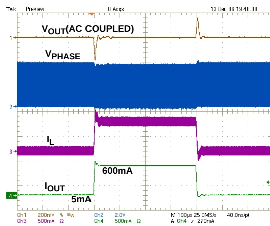
FIGURE 10. LOAD TRANSIENT (PWM, V_{\text{IN}} = 3.6\text{V} , V_{\text{OUT}} = 1.6\text{V} )
