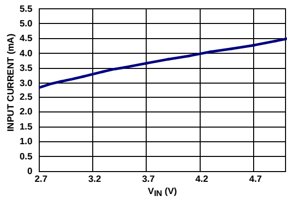
FIGURE 6. I_Q vs V_{\text{IN}} (PWM)
