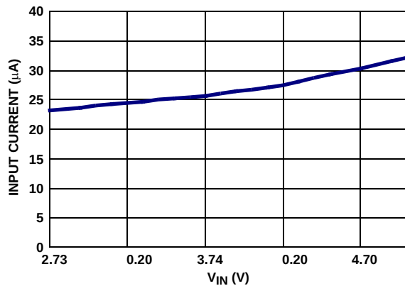
FIGURE 5. I_Q vs V_{\text{IN}} (PFM)
