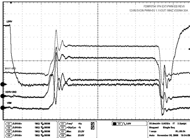
Figure 5. FDMF6704
