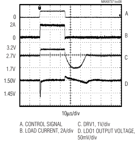
LOAD TRANSIENT (NO LOAD TO 2A)
