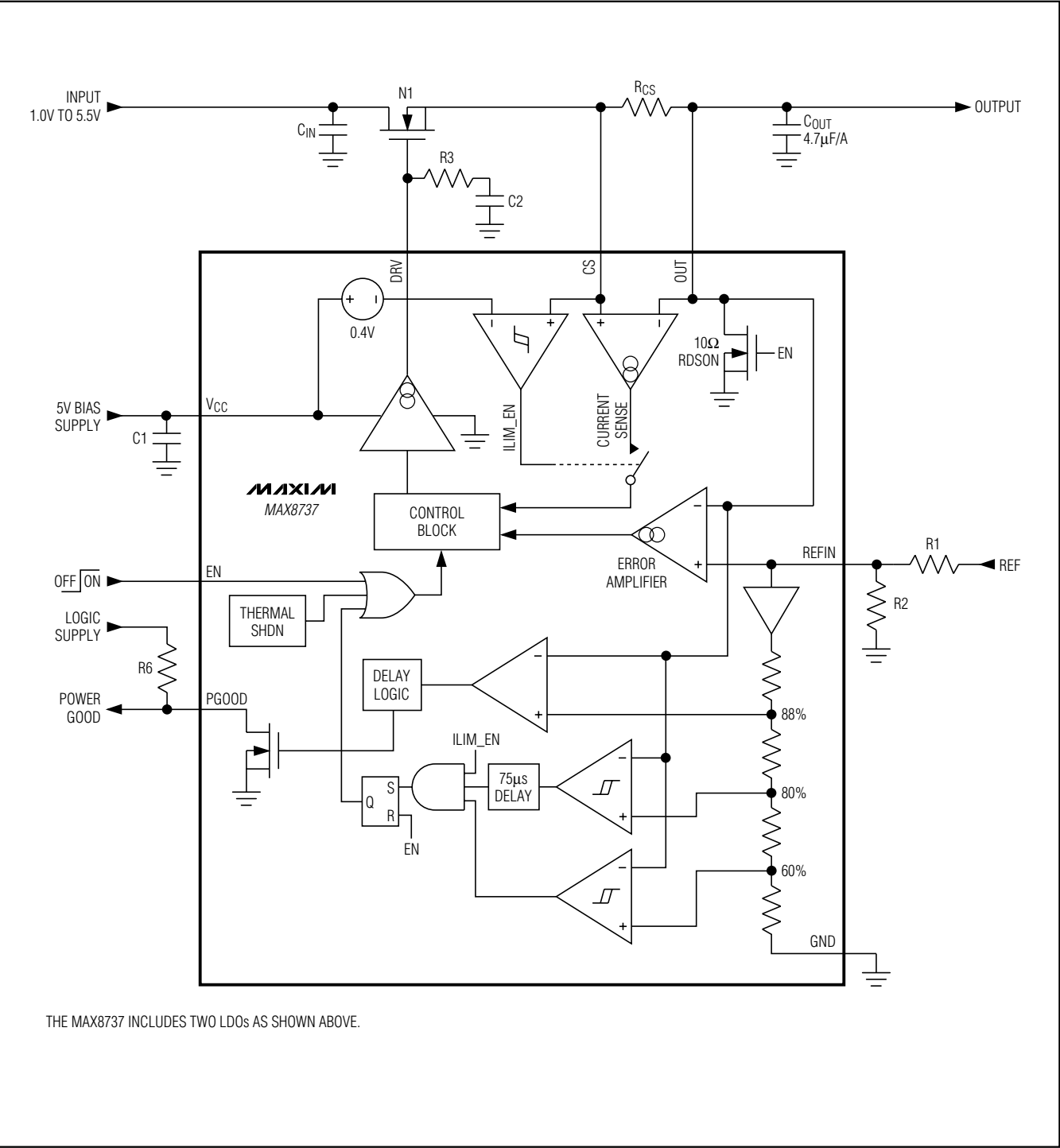
Figure 2. Functional Diagram
