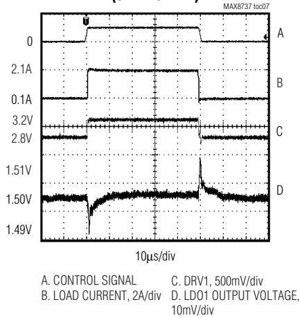
LOAD TRANSIENT (0.1A TO 2.1A)
