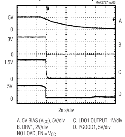
SOFT-STOP (UVLO FALLING EDGE)
