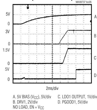
SOFT-START (UVLO RISING EDGE)
