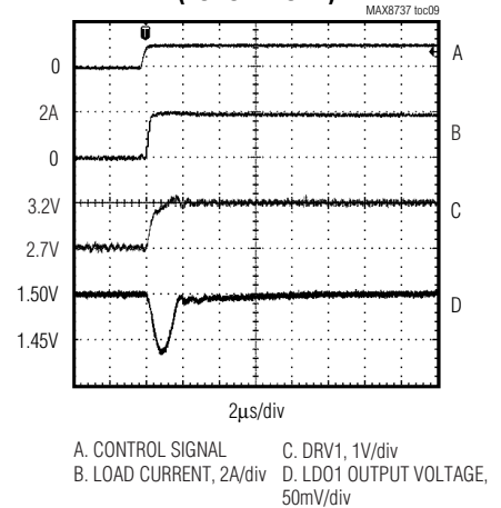
LOAD TRANSIENT (NO LOAD TO 2A)
