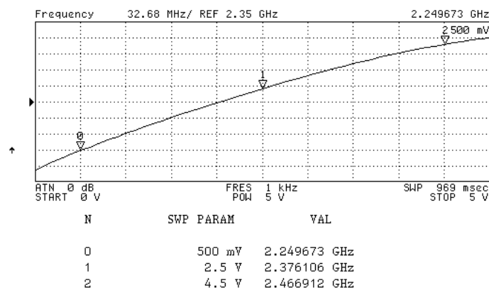
Tuning Curve (Typical)
