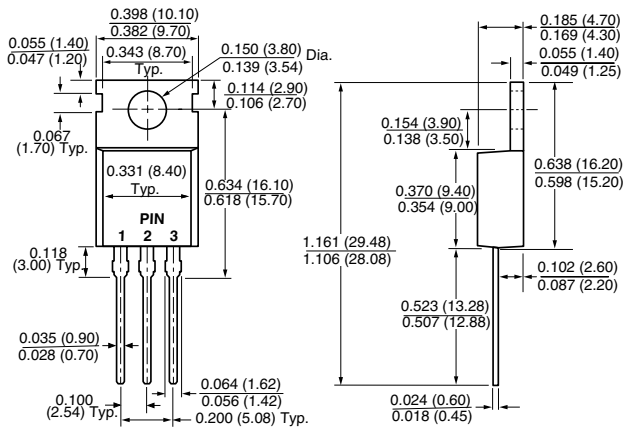
TO-220AB
