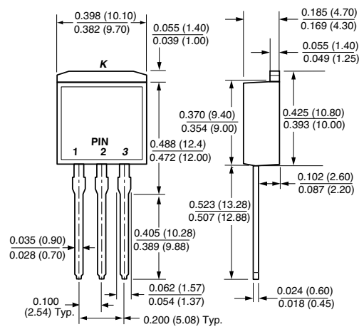
TO-262AA
