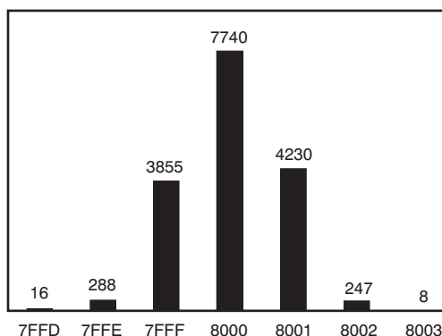
Figure 43. Histogram of 16,384 Conversions with V_{IN} = 0 V in \pm 10 V Bipolar Range
