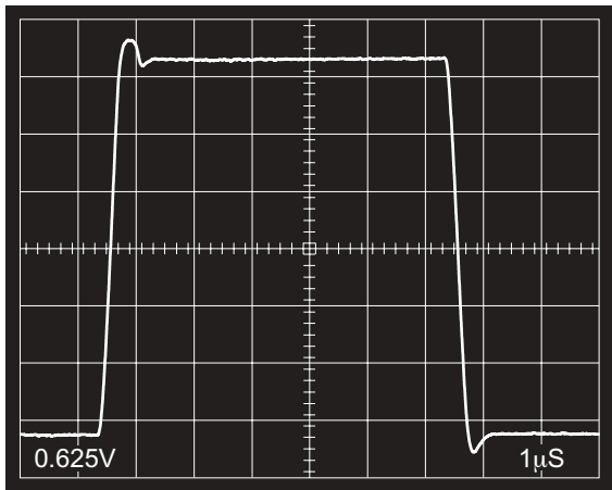
Large-Signal Response
