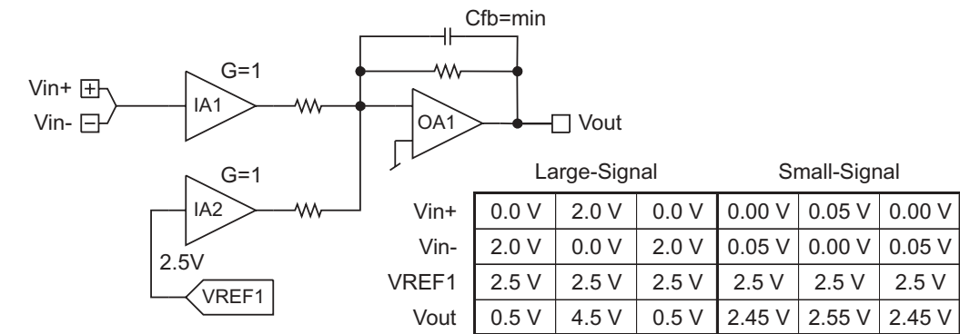
Step Response Setup Diagram
