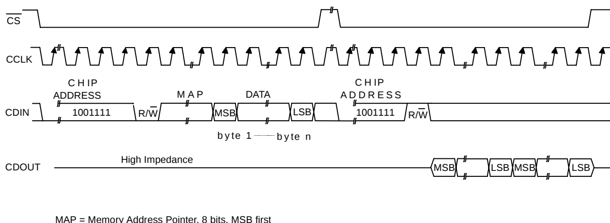
Figure 22. Software Mode Timing, SPI Mode
