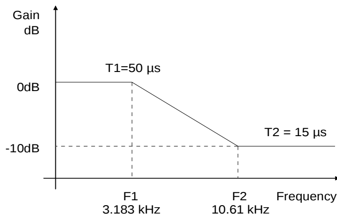
Figure 17. De-Emphasis Curve
