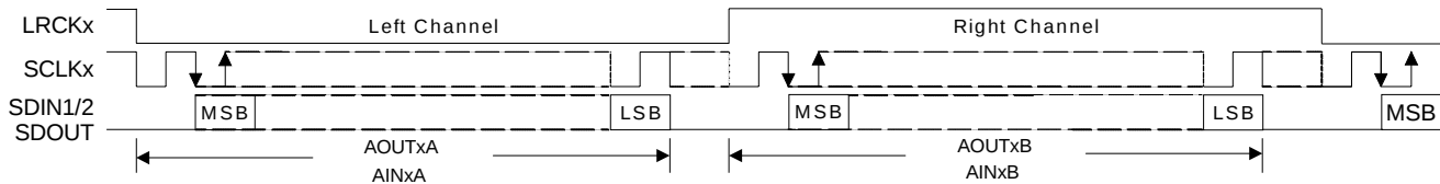
Figure 14. I 2 S up to 24-Bit Data
