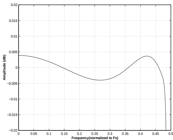
Figure 34. Single-Speed Passband Ripple
