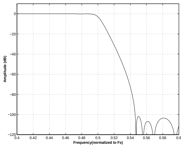
Figure 32. Single-Speed Transition Band
