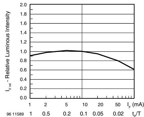
Figure 9. Rel. Luminous Intensity vs. Forward Current/Duty Cycle
