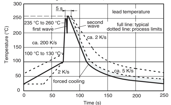
Figure 11. Double Wave Soldering of Opto Devices (all Packages)
