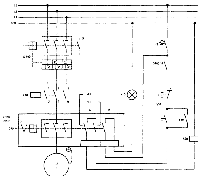
Safety switch with load shedding and signalling N switch-disconnector (example)
