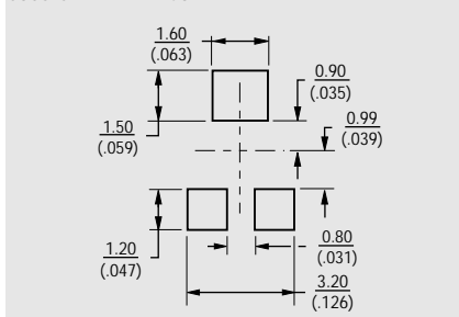
SUGGESTED PWB LAYOUT
