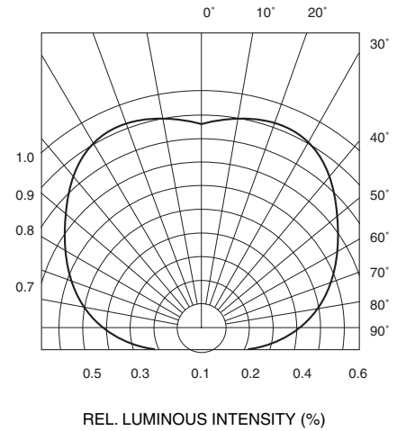
Fig. 4 Radiation Diagram
