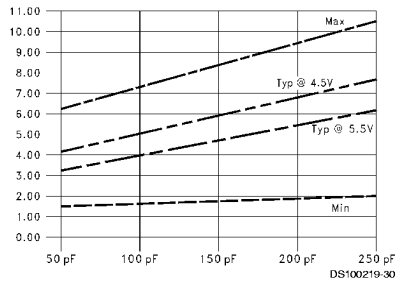
T_{PZH} vs Load Capacitance T_A = 25^\circ\text{C} , 8 Outputs Switching, OE to Output
