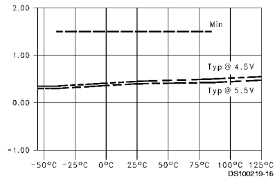
T_{SET} LOW vs Temperature ( T_A ), C_L = 50 pF, 1 Output Switching, Data to LE
