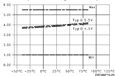
T_{PLZ} vs Temperature ( T_A ), C_L = 50 pF, 8 Outputs Switching, OE to Output
