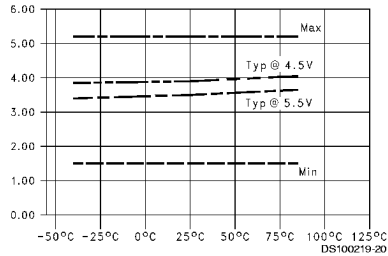
T_{PLH} vs Temperature ( T_A ), C_L = 50 pF, 8 Outputs Switching, Data to Output
