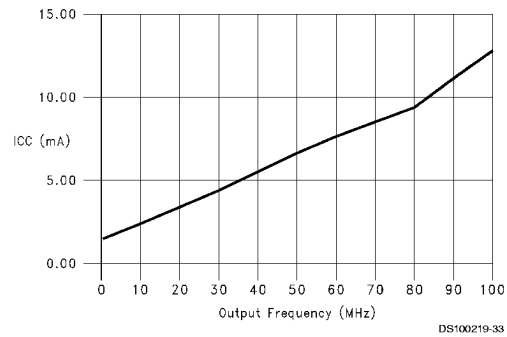
Typical I_{CC} vs Output Switching Frequency, C_L = 0 pF, V_{CC} = V_{IH} = 5.5\text{V} , LE = GND, 1 Output Switching at 50% Duty Cycle, Data to Output, Transparent Mode with Unused Data Inputs = V_{IH}
