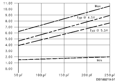
T_{PZL} vs Load Capacitance T_A = 25^\circ\text{C} , 8 Outputs Switching, OE to Output
