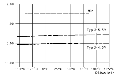
T_{SET} HIGH vs Temperature ( T_A ), C_L = 50 pF, 1 Output Switching, Data to LE
