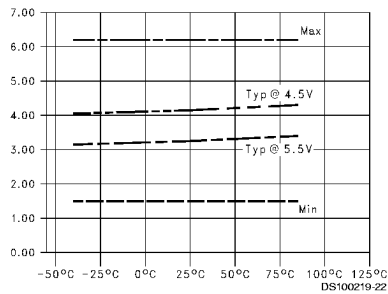
T_{PZH} vs Temperature ( T_A ), C_L = 50 pF, 8 Outputs Switching, OE to Output
