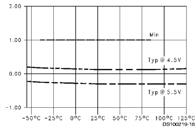
T_{HOLD} HIGH vs Temperature ( T_A ), C_L = 50 pF, 1 Output Switching, Data to LE
