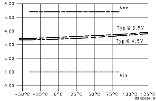
T_{PLZ} vs Temperature ( T_A ), C_L = 50 pF, 1 Output Switching, OE to Output
