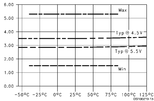
T_{PZL} vs Temperature ( T_A ), C_L = 50 pF, 1 Output Switching, OE to Output
