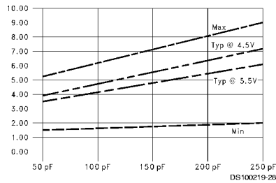
T_{PLH} vs Load Capacitance T_A = 25^\circ\text{C} , 8 Outputs Switching, Data to Output
