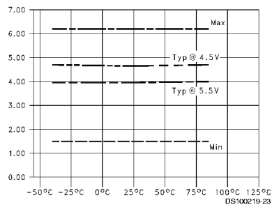
T_{PZL} vs Temperature ( T_A ), C_L = 50 pF, 8 Outputs Switching, OE to Output
