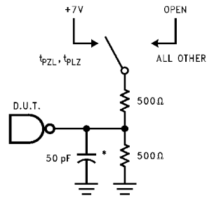
FIGURE 1. Test Load
