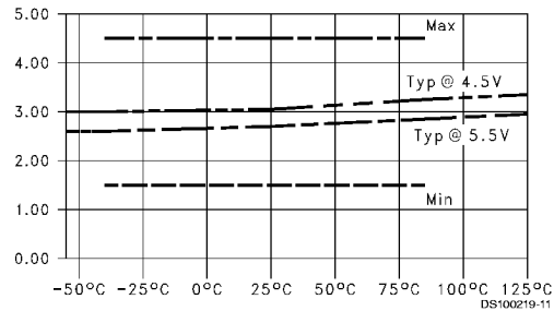
T_{PHL} vs Temperature ( T_A ), C_L = 50 pF, 1 Output Switching, Data to Output
