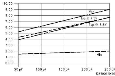
T_{PHL} vs Load Capacitance T_A = 25^\circ\text{C} , 8 Outputs Switching, Data to Output
