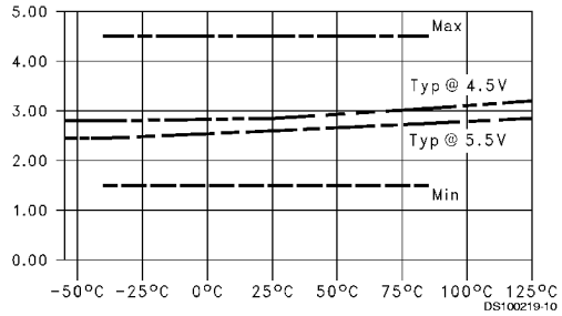
T_{PLH} vs Temperature ( T_A ), C_L = 50 pF, 1 Output Switching, Data to Output
