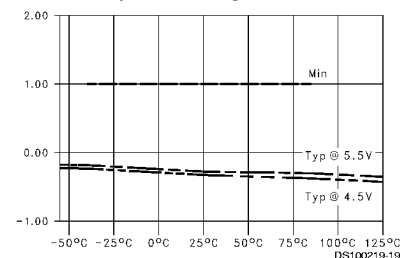
T_{HOLD} LOW vs Temperature ( T_A ), C_L = 50 pF, 1 Output Switching, Data to LE
