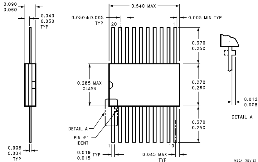
20-Lead Ceramic Flatpack NS Package Number W20A
