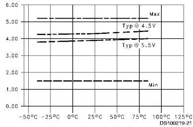
T_{PHL} vs Temperature ( T_A ), C_L = 50 pF, 8 Outputs Switching, Data to Output
