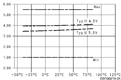
T_{PHZ} vs Temperature ( T_A ), C_L = 50 pF, 8 Outputs Switching, OE to Output
