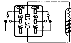
Terminal Arrangement (Bottom View)
