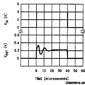
Start-Up Response
