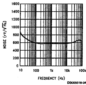
Noise Voltage
